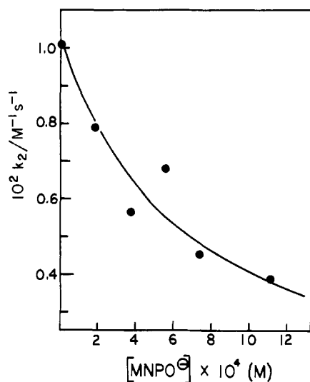
Figure 1. The observed second-order rate constants for the reaction of 3-chloroquinclidine with m -nitrophenyl phenyl carbonate in the presence of added m -nitrophenoxide ion (MNPO - ). The solid line is calculated from eq 2 with k_{-1}/k_2 = 10^{3.2} \text{ M}^{-1} . The rates were measured at 25 °C, ionic strength 1.0 M maintained with tetramethylammonium chloride, [3\text{-Cl-Q}]_{\text{free base}} = 0.04 \text{ M} , pH 9.01.
